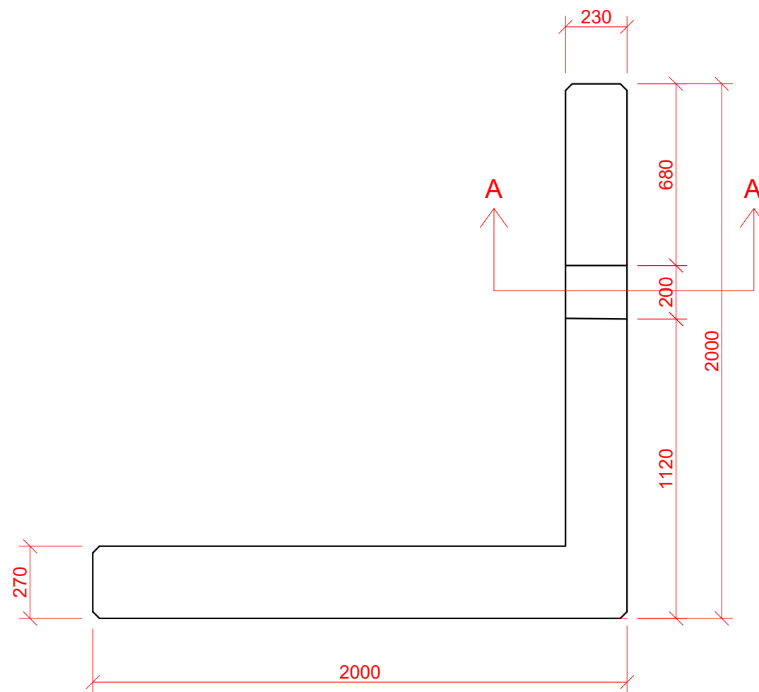
Betongplan
